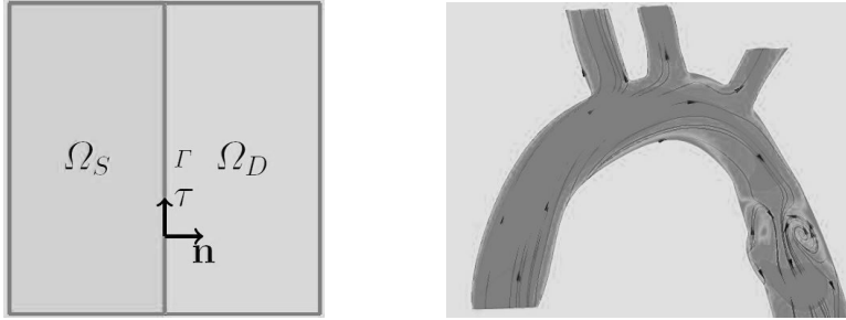
Figure 1: Darcy-Stokes system: model problem with simple geometry (left); realistic problem with more complicated geometry of the interface
