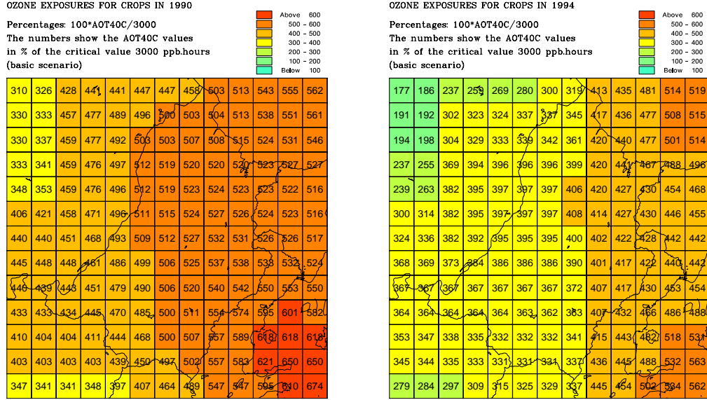
Fig. 1. AOT40 maps of Bulgarian region for 1990 and 1994.
