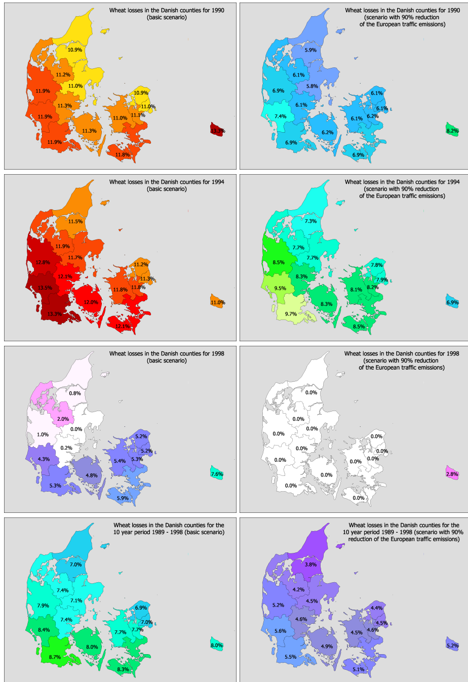
Fig. 2. Wheat losses in the Danish regions under the Basic scenario (left plots) and the Traffic scenario (right plots) for 1990, 1994, 1998, and the average losses for the period 1989–98
